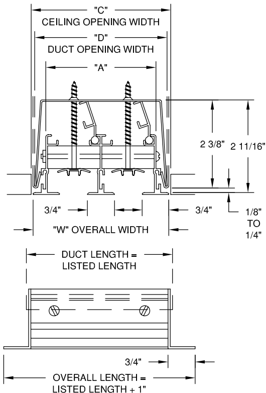
MODEL - 9475-672 WITH HANGER BRACKET
